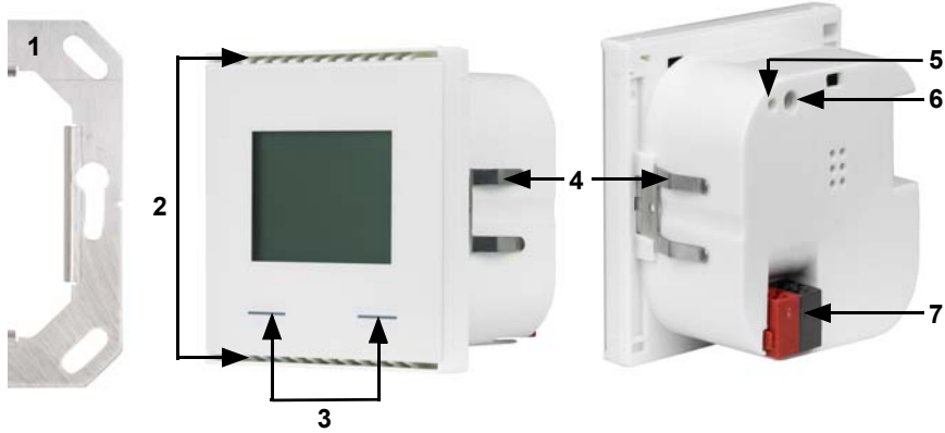
Fig. 2 1 Base plate 2 Openings for air circulation 3 Touch sensitive buttons 4 Catches 5 Programming LED (recessed) 6 Programming button (recessed) for teaching device
