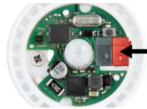
Fig. 8 Plug the KNX terminal with the bus cable to the slot.
