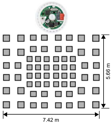
Fig. 1 Distance 2.50 m
