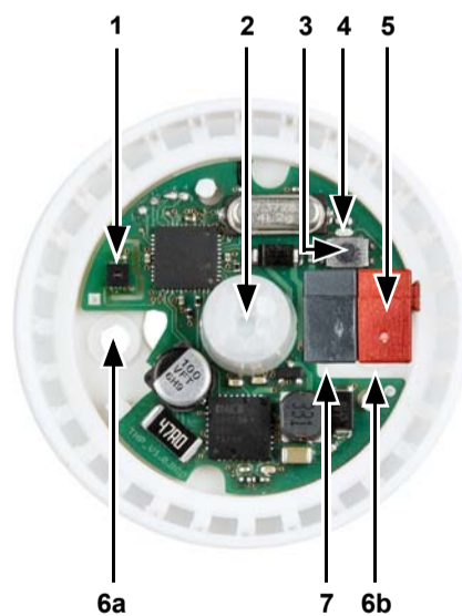
Fig. 4 1 Sensors for temperature, humidity 2 Motion sensor 3 Programming button 4 Programming LED 5 KNX terminal BUS +/- 6 a+b Holes for mounting (hole distance 30 mm) 7 Cable bushing (under the KNX terminal)
