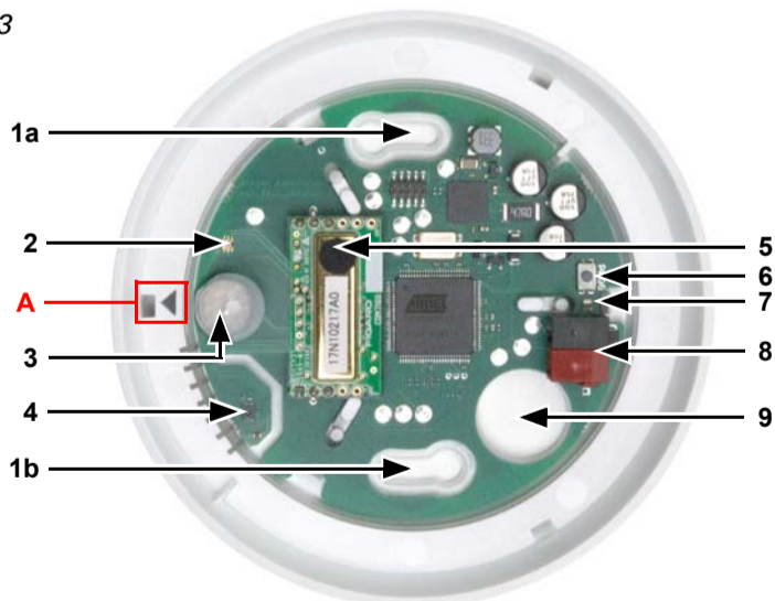
1 a+b Long holes for mounting (hole distance 60 mm) 2 Brightness sensor 3 Motion sensor 4 Sensors for temperature, humidity, pressure 5 CO 2 sensor 6 Programming button 7 Programming LED 8 KNX-terminal BUS +/- 9 Cable bushing A Mark for aligning the cover
