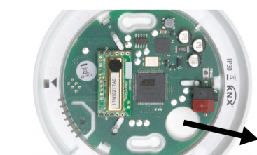
Fig. 4 Lead the bus cable through the cable bushing in the skirting.
