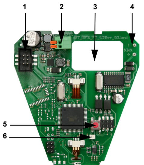
Fig. 13 1 Slot for cable connection to the rain sensor in the housing cover 2 Tension clamp for voltage supply (20...32 V DC). Massive conductors of up to 1.5 mm 2 or conductors with fine wires. Terminal configuration independent from polarity (+/- or -/+). 3 Opening for the cable for the voltage supply and for bus cable 4 Slot for KNX clamp +/- 5 Programming pushbutton for the teach-in of the device 6 Programming LED
