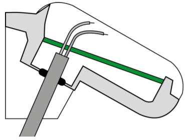
Fig. 11 Remove the cable shielding under the circuit board and only feed the connector cables upwards through the openings in the circuit board.
